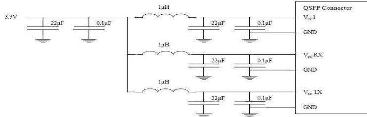
Figure1. Host Board Power Supply Filtering
